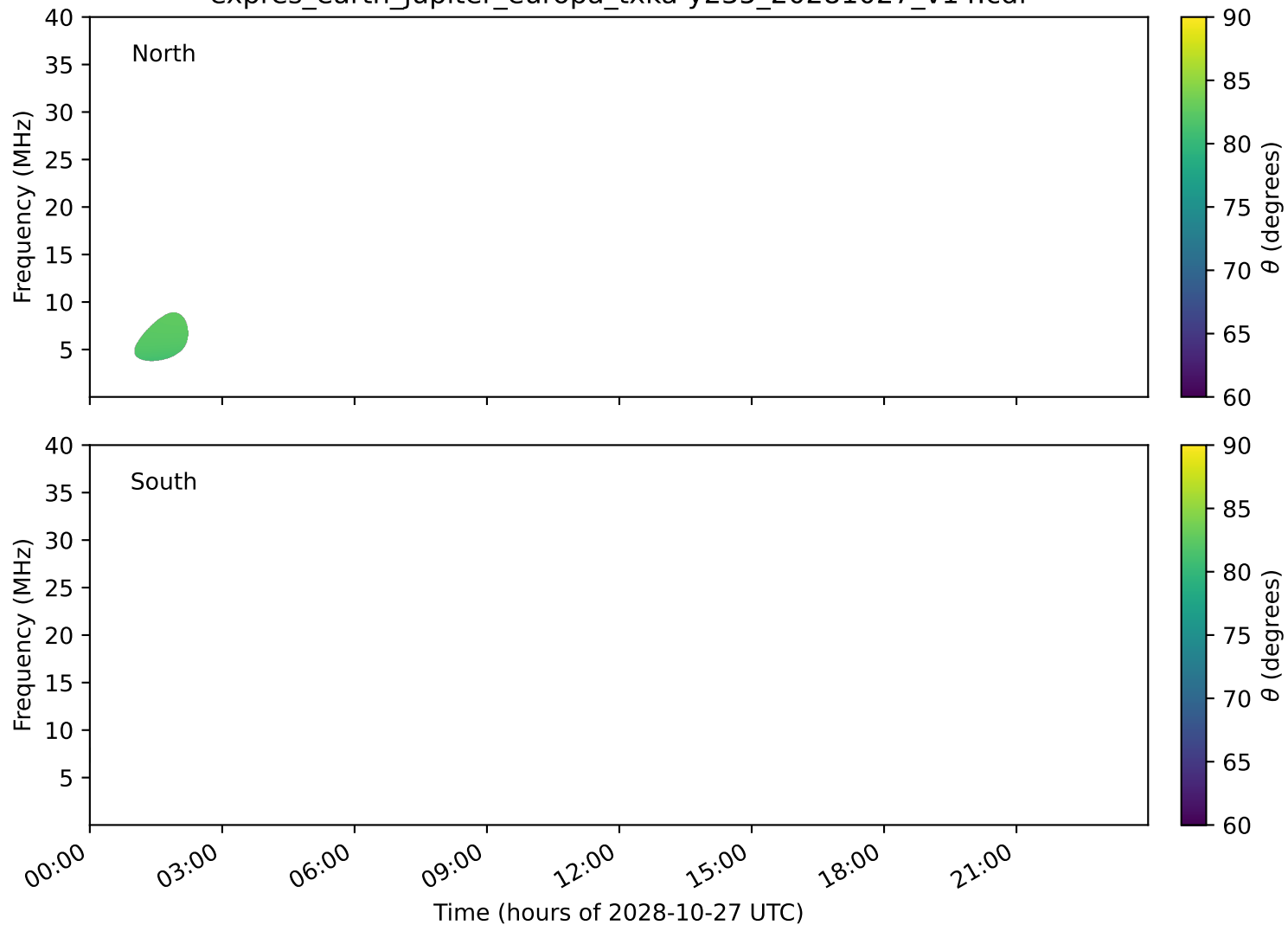
expres_earth_jupiter_europa_txka-y235_20281027_v14.cdf
