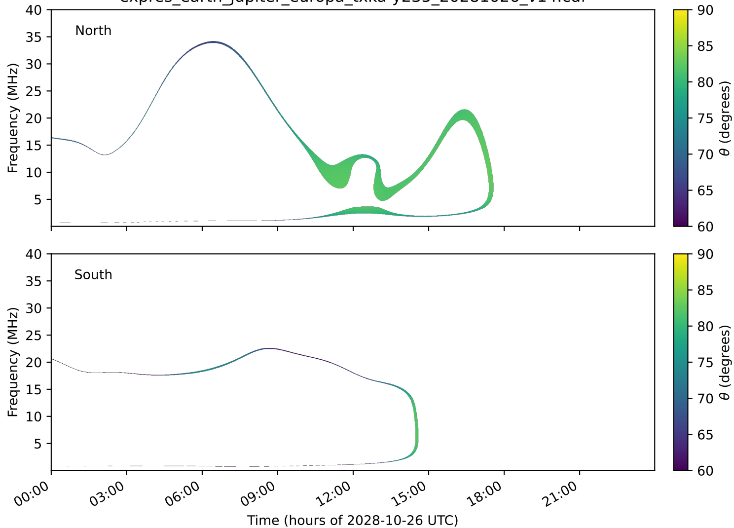
expres_earth_jupiter_europa_txka-y235_20281026_v14.cdf
