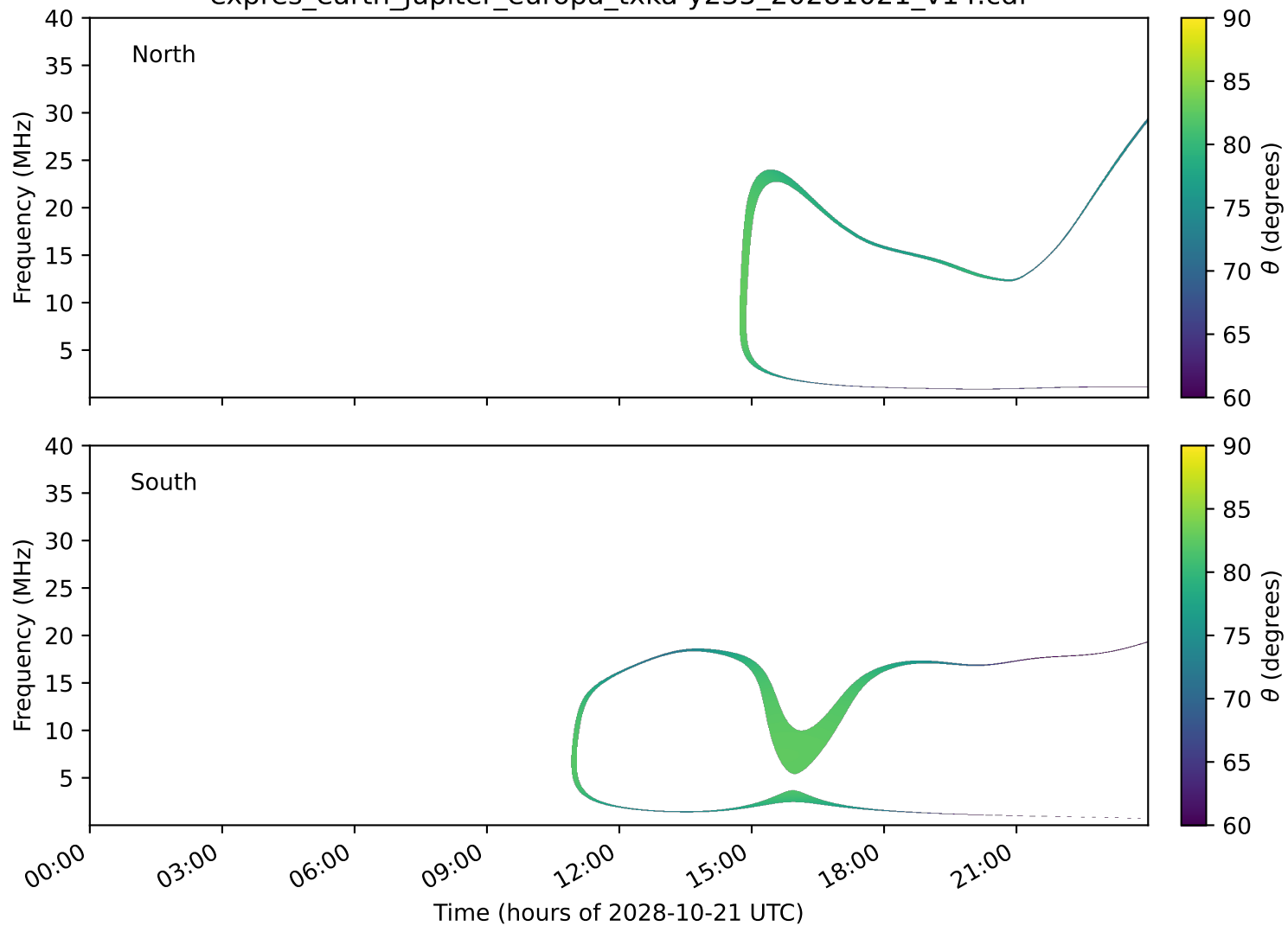
expres_earth_jupiter_europa_txka-y235_20281021_v14.cdf
