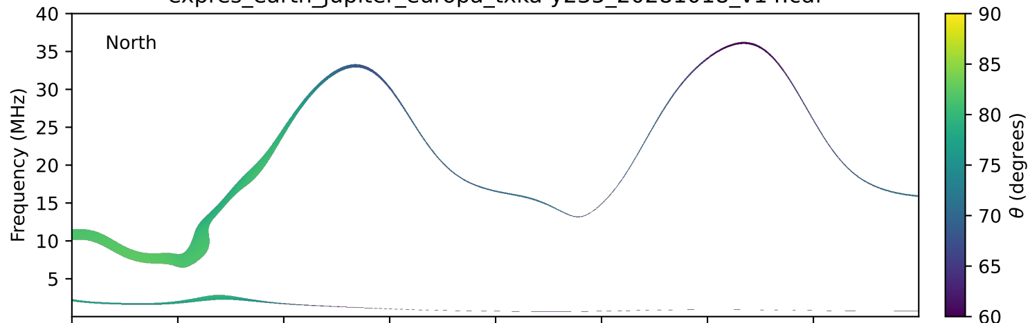
expres_earth_jupiter_europa_txka-y235_20281018_v14.cdf
