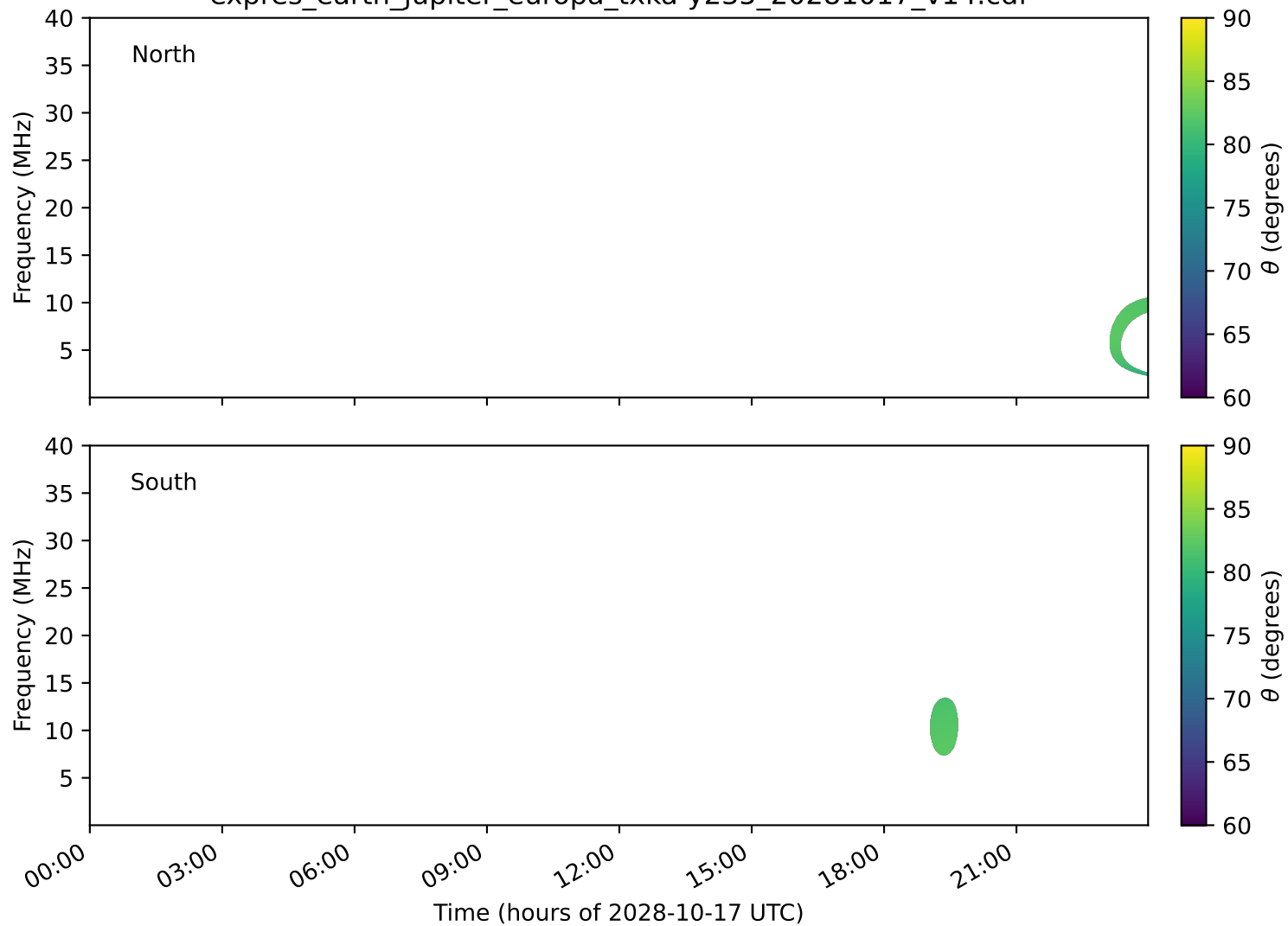
expres_earth_jupiter_europa_txka-y235_20281017_v14.cdf
