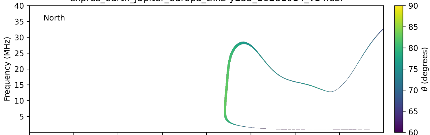
expres_earth_jupiter_europa_txka-y235_20281014_v14.cdf
