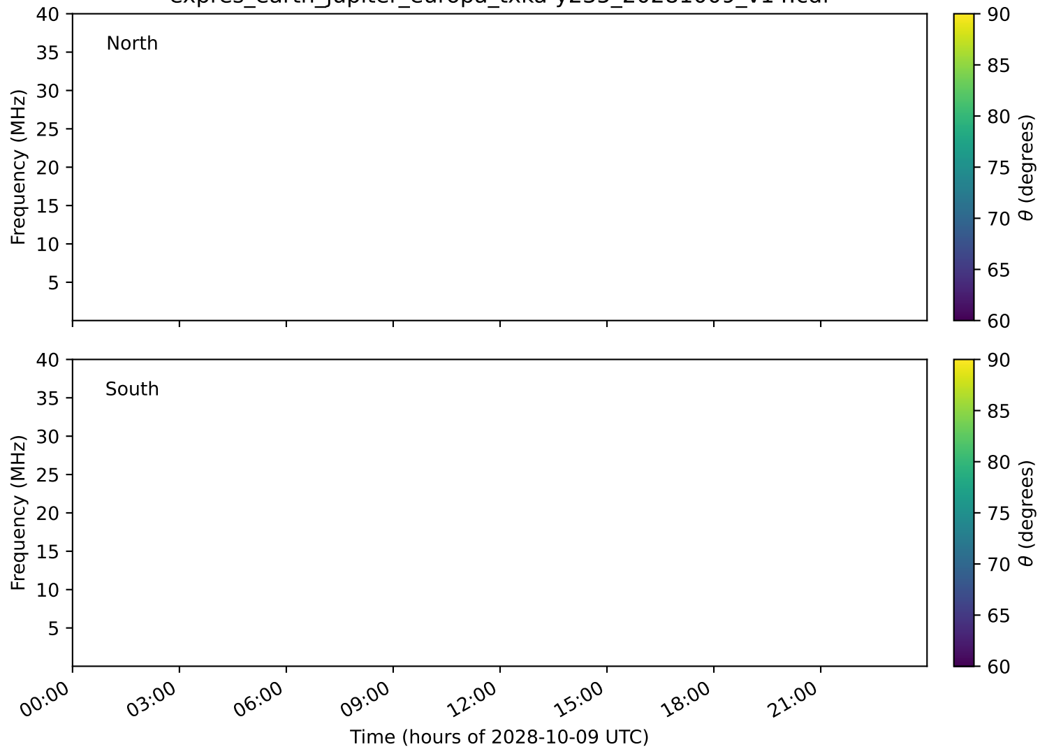
expres_earth_jupiter_europa_txka-y235_20281009_v14.cdf
