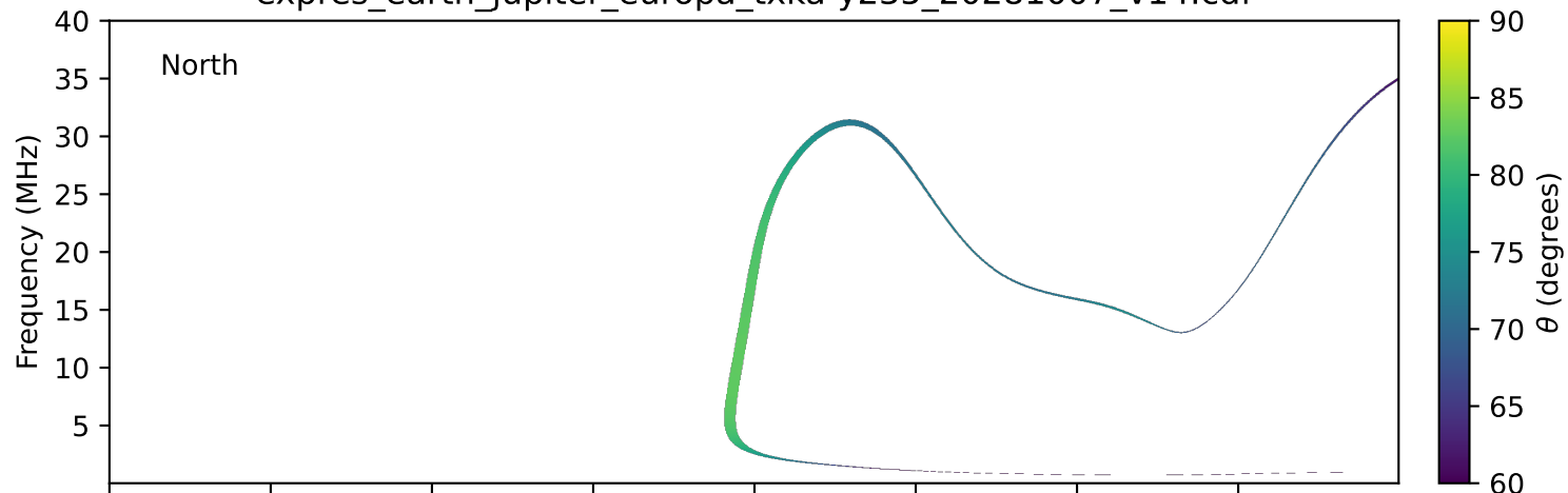
expres_earth_jupiter_europa_txka-y235_20281007_v14.cdf
