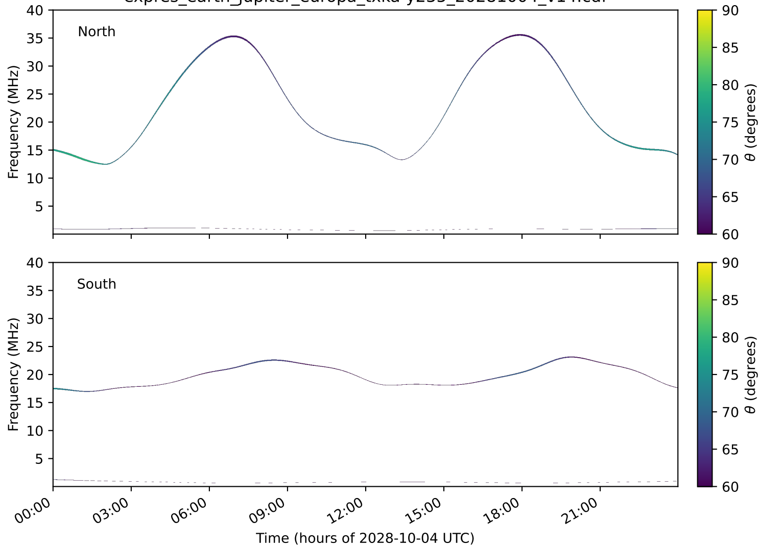
expres_earth_jupiter_europa_txka-y235_20281004_v14.cdf
