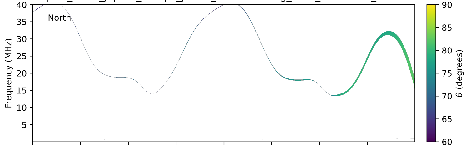
expres_earth_jupiter_europa_jrm33_lossc-wid1deg_3kev_20281015_v11.cdf
