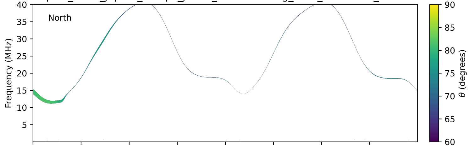
expres_earth_jupiter_europa_jrm33_lossc-wid1deg_3kev_20281004_v11.cdf
