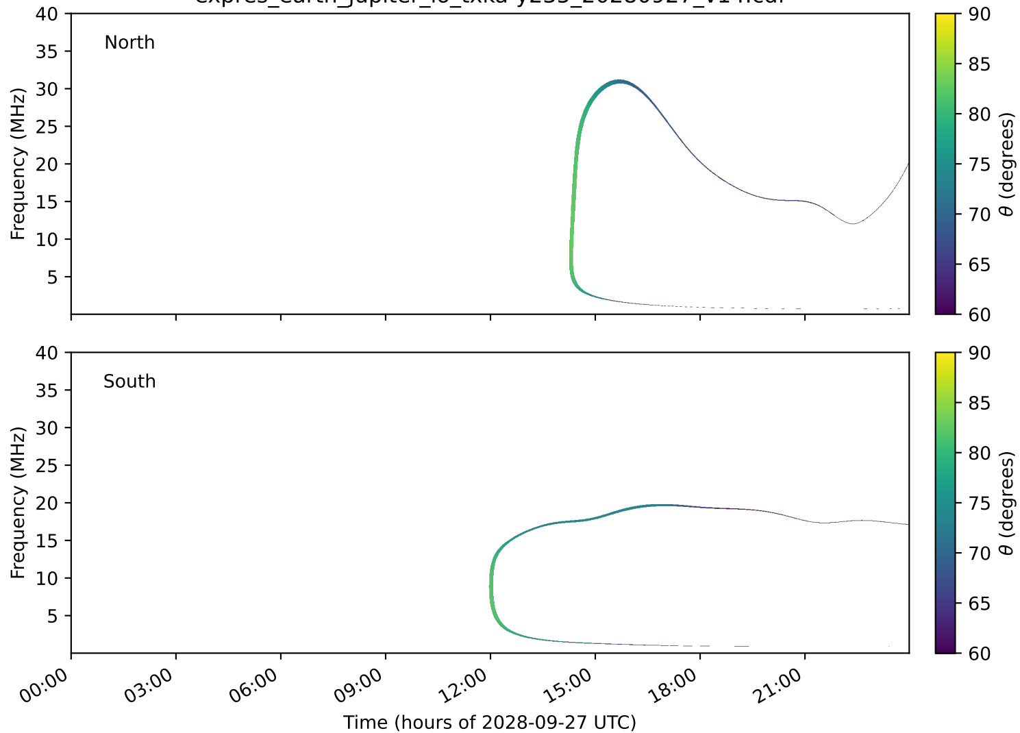
expres_earth_jupiter_io_txka-y235_20280927_v14.cdf
