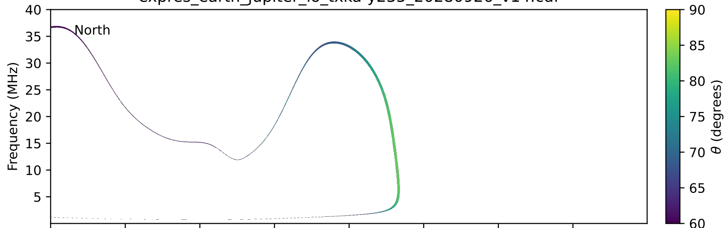
expres_earth_jupiter_io_txka-y235_20280926_v14.cdf
