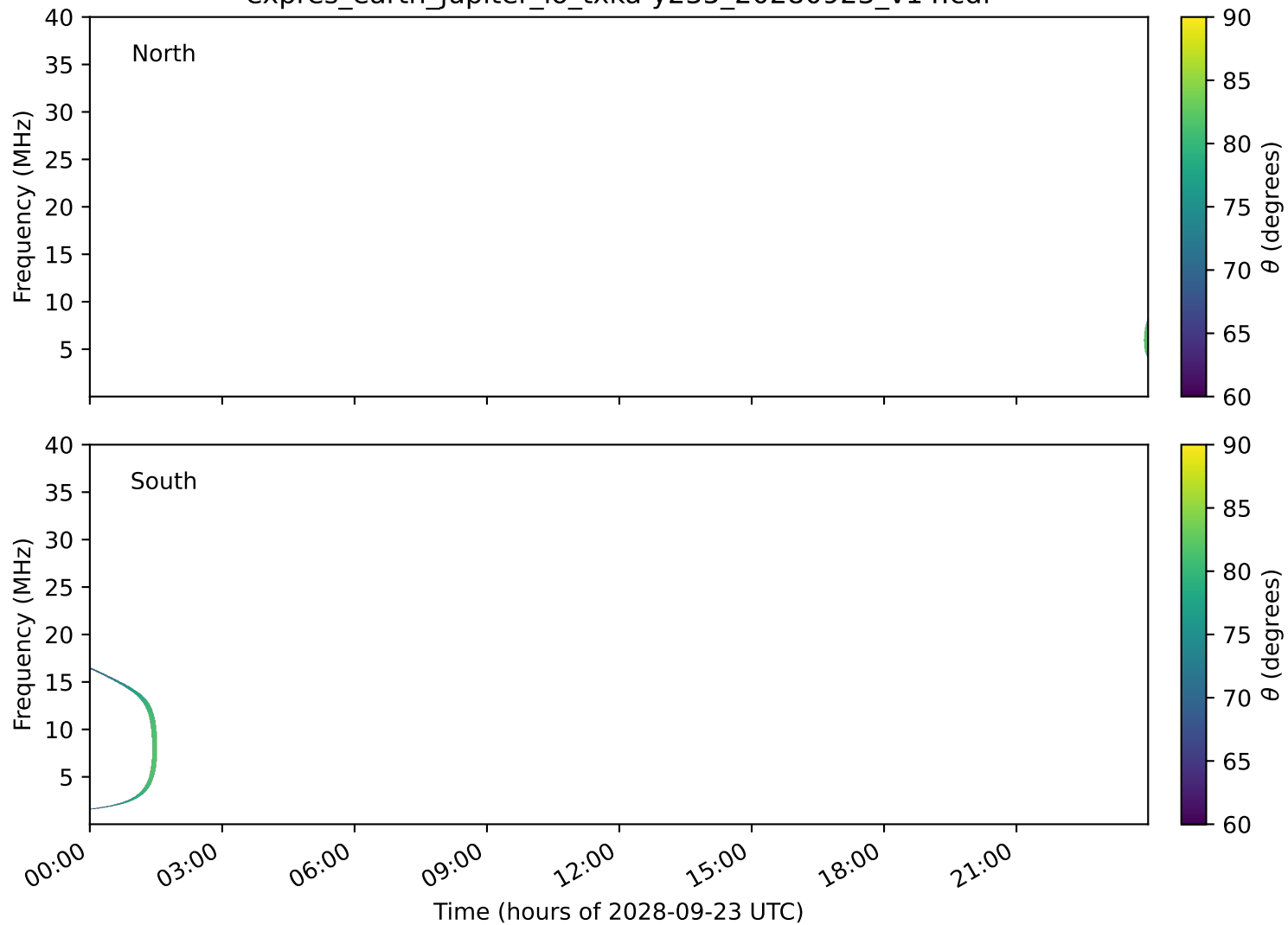
expres_earth_jupiter_io_txka-y235_20280923_v14.cdf
