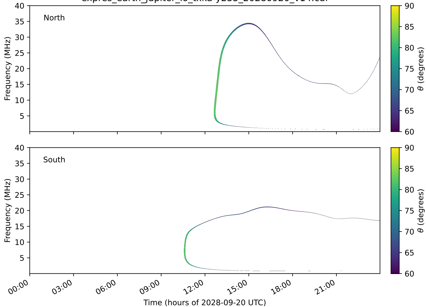
expres_earth_jupiter_io_txka-y235_20280920_v14.cdf
