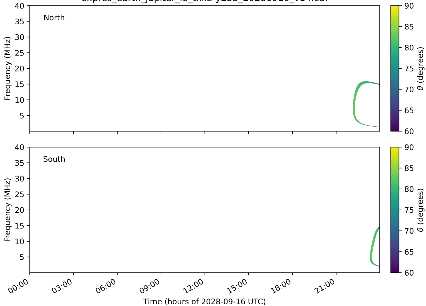
expres_earth_jupiter_io_txka-y235_20280916_v14.cdf
