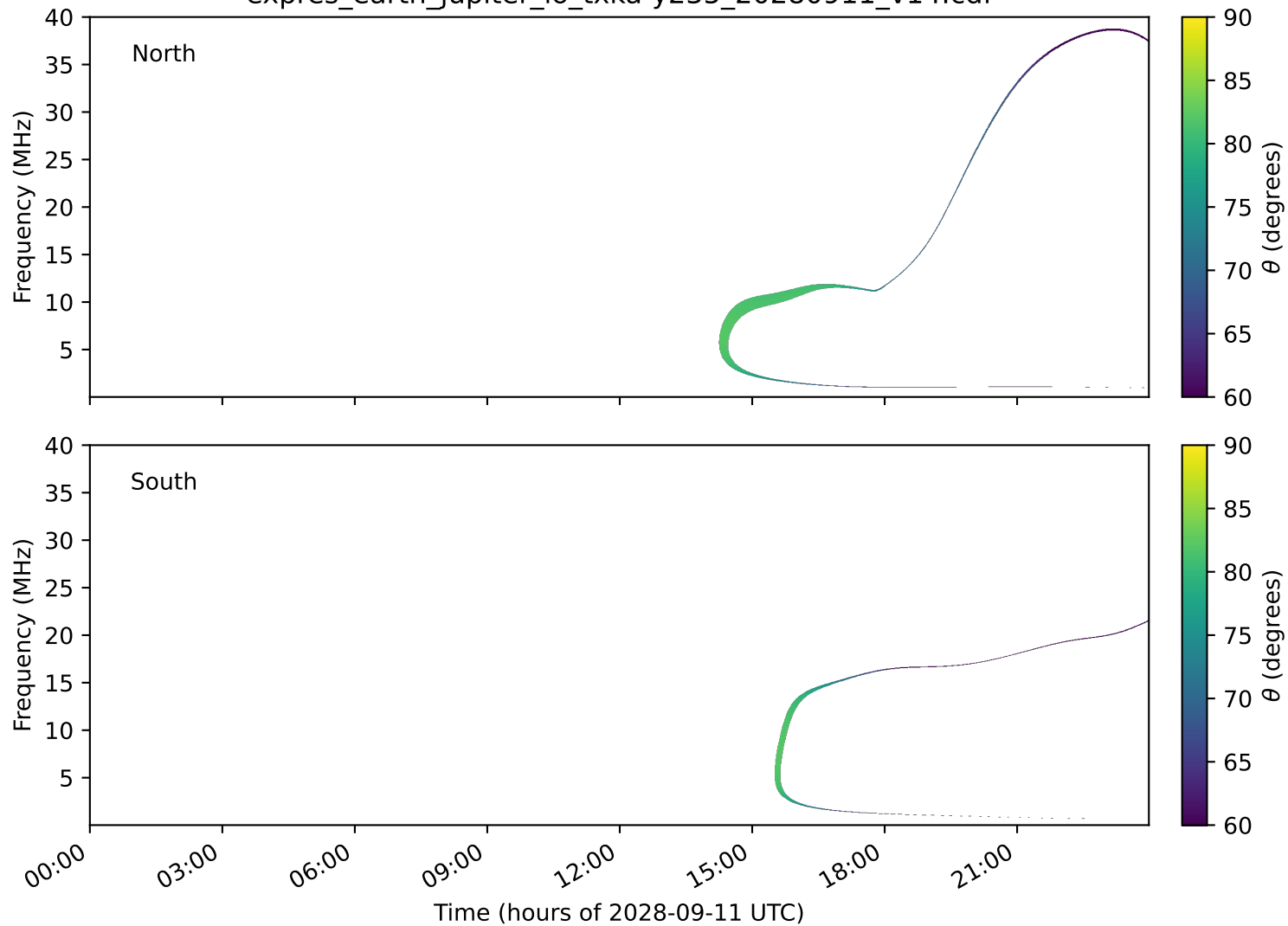
expres_earth_jupiter_io_txka-y235_20280911_v14.cdf
