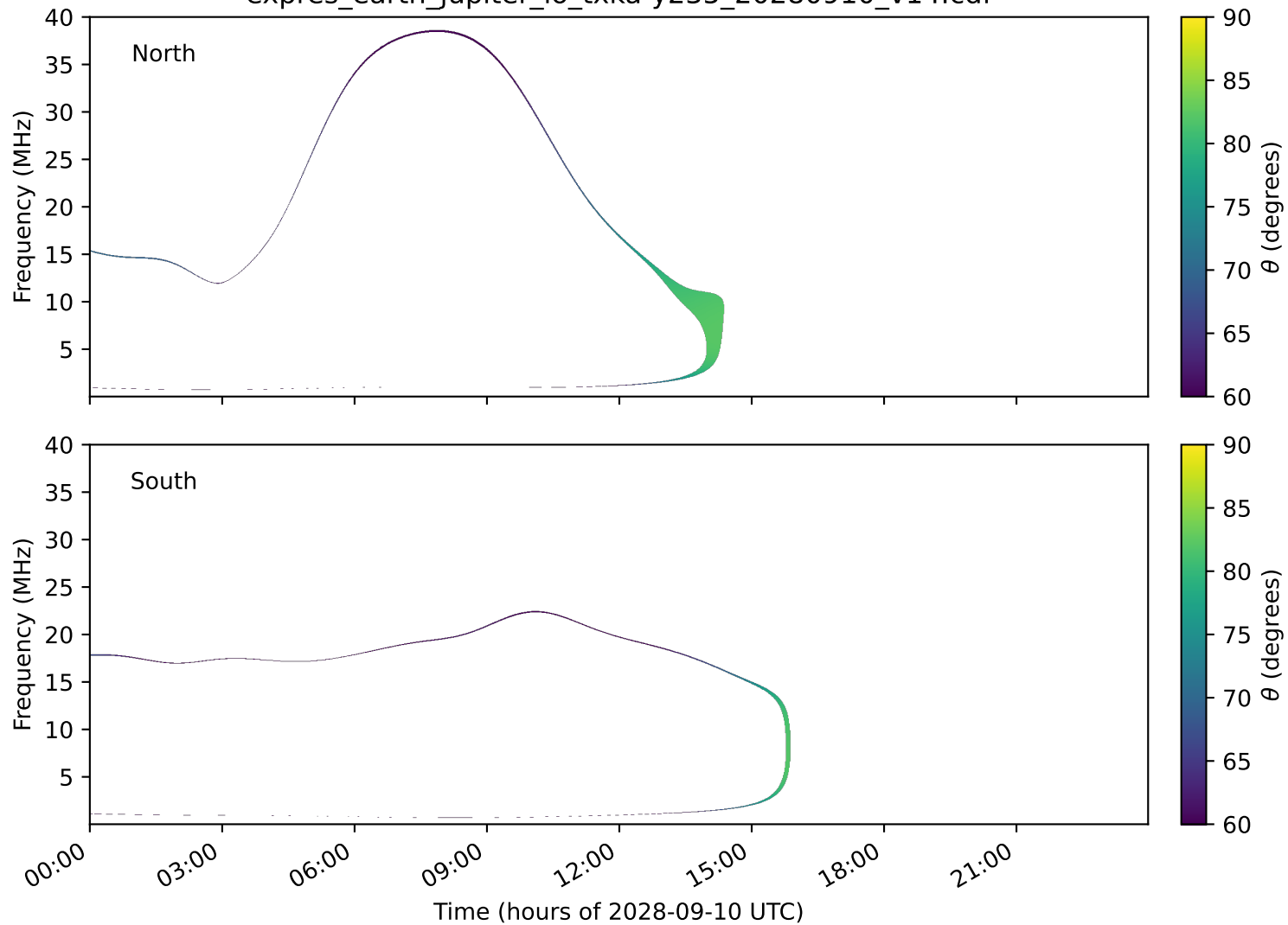
expres_earth_jupiter_io_txka-y235_20280910_v14.cdf
