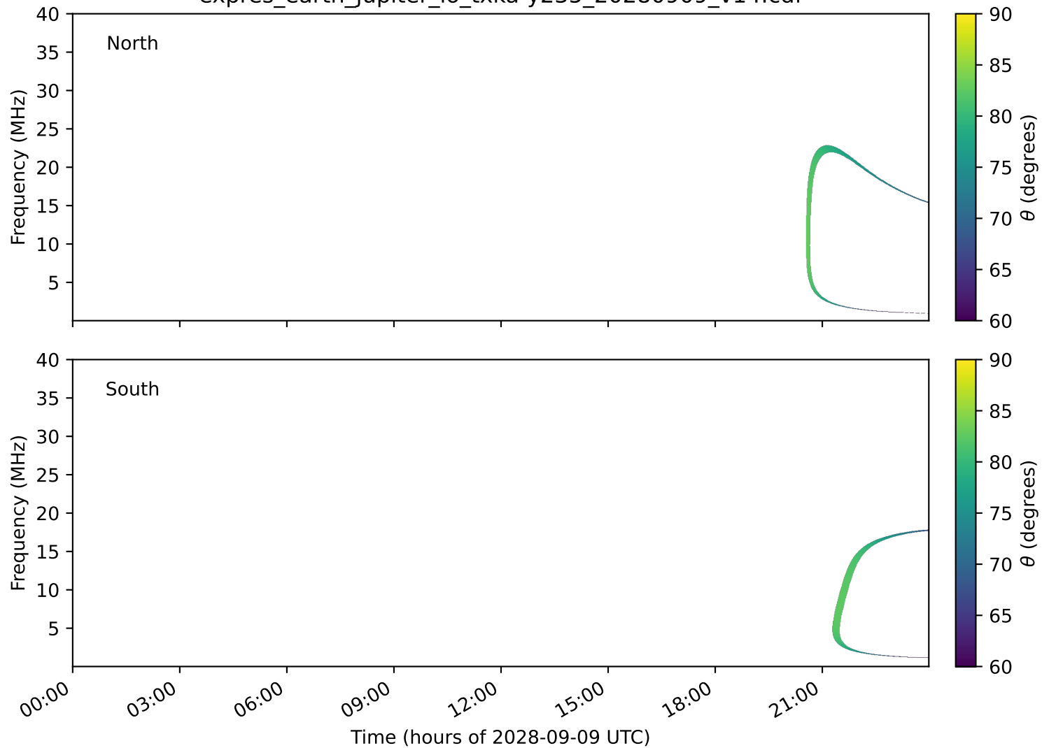
expres_earth_jupiter_io_txka-y235_20280909_v14.cdf
