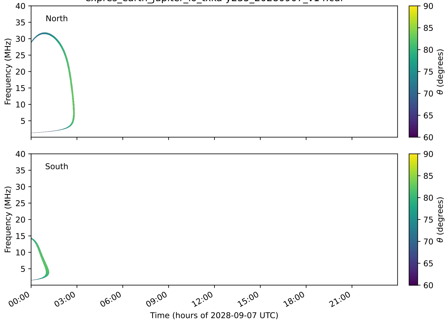
expres_earth_jupiter_io_txka-y235_20280907_v14.cdf
