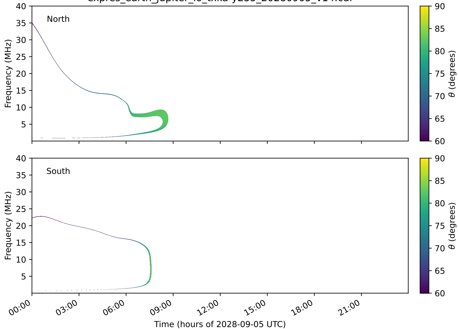
expres_earth_jupiter_io_txka-y235_20280905_v14.cdf
