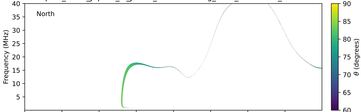
expres_earth_jupiter_io_jrm33_lossc-wid1deg_3kev_20280929_v11.cdf
