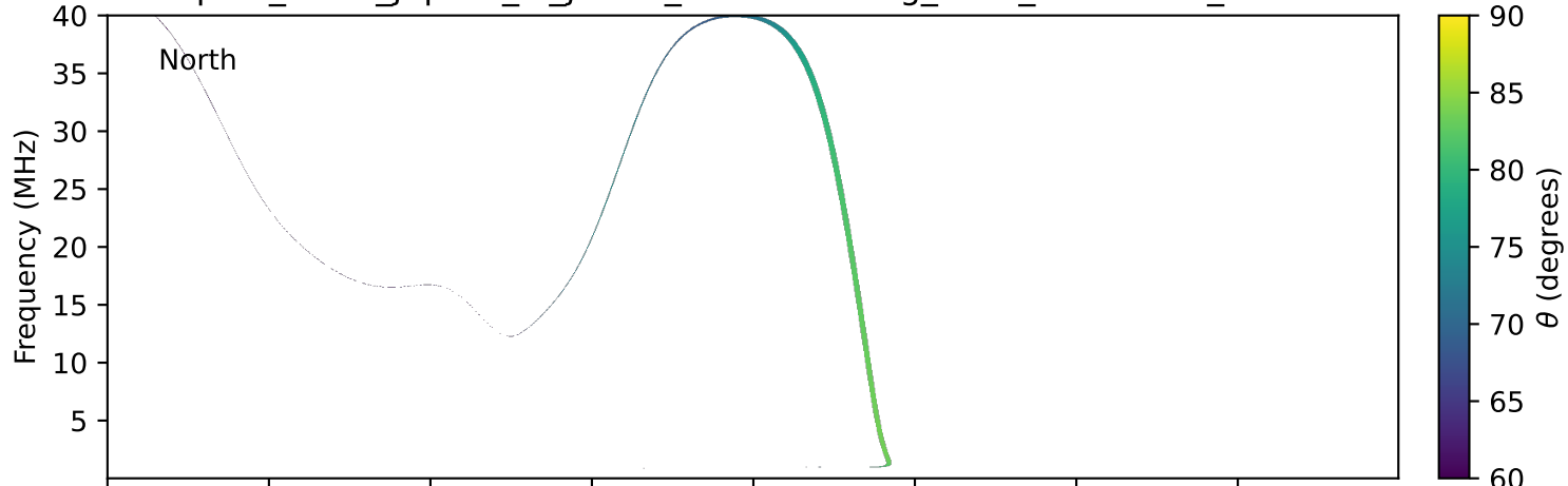
expres_earth_jupiter_io_jrm33_lossc-wid1deg_3kev_20280926_v11.cdf
