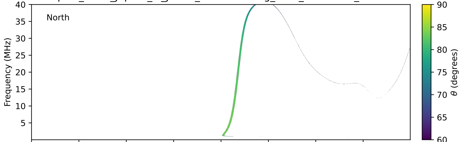
expres_earth_jupiter_io_jrm33_lossc-wid1deg_3kev_20280920_v11.cdf
