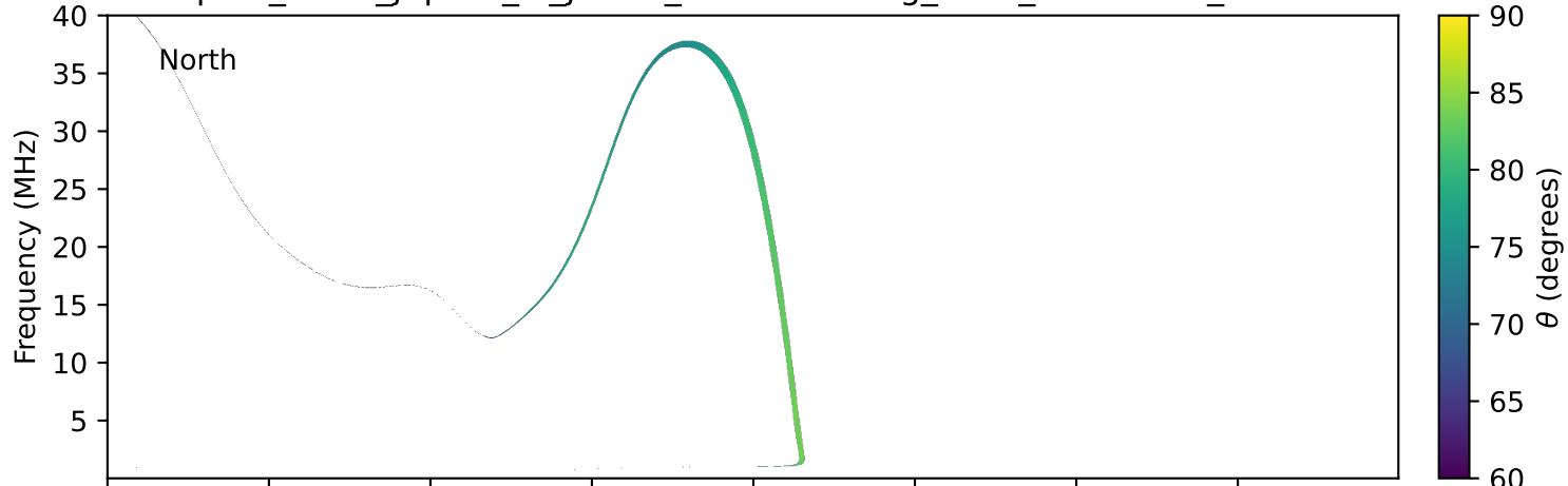
expres_earth_jupiter_io_jrm33_lossc-wid1deg_3kev_20280919_v11.cdf
