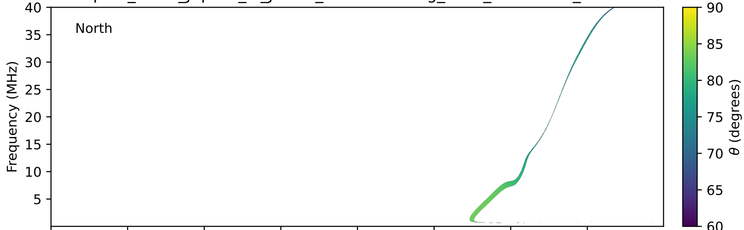
expres_earth_jupiter_io_jrm33_lossc-wid1deg_3kev_20280918_v11.cdf
