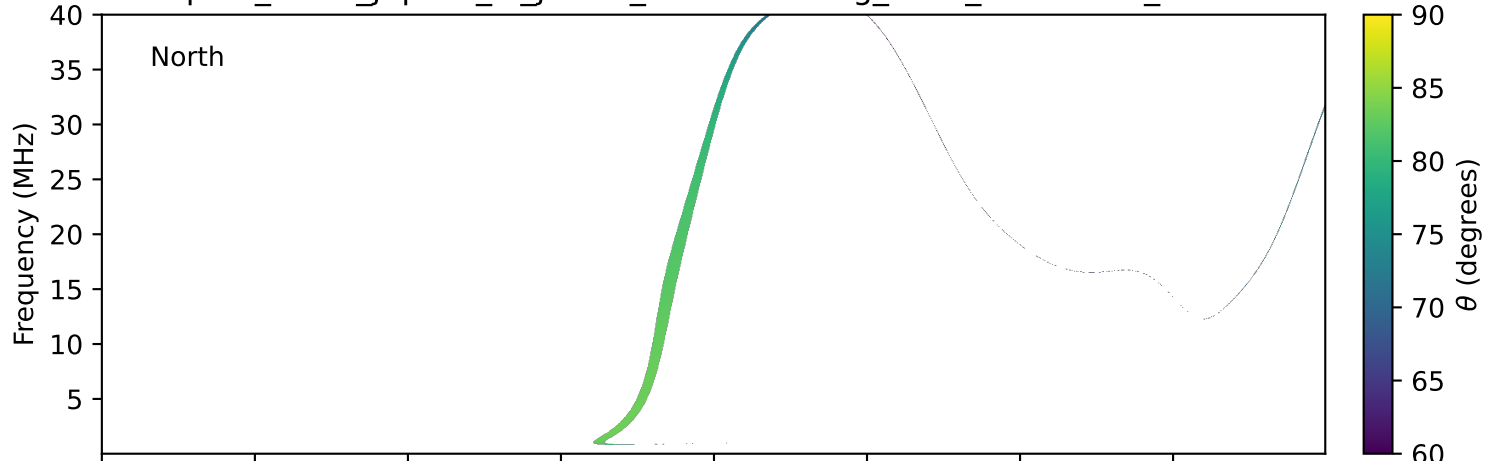
expres_earth_jupiter_io_jrm33_lossc-wid1deg_3kev_20280913_v11.cdf
