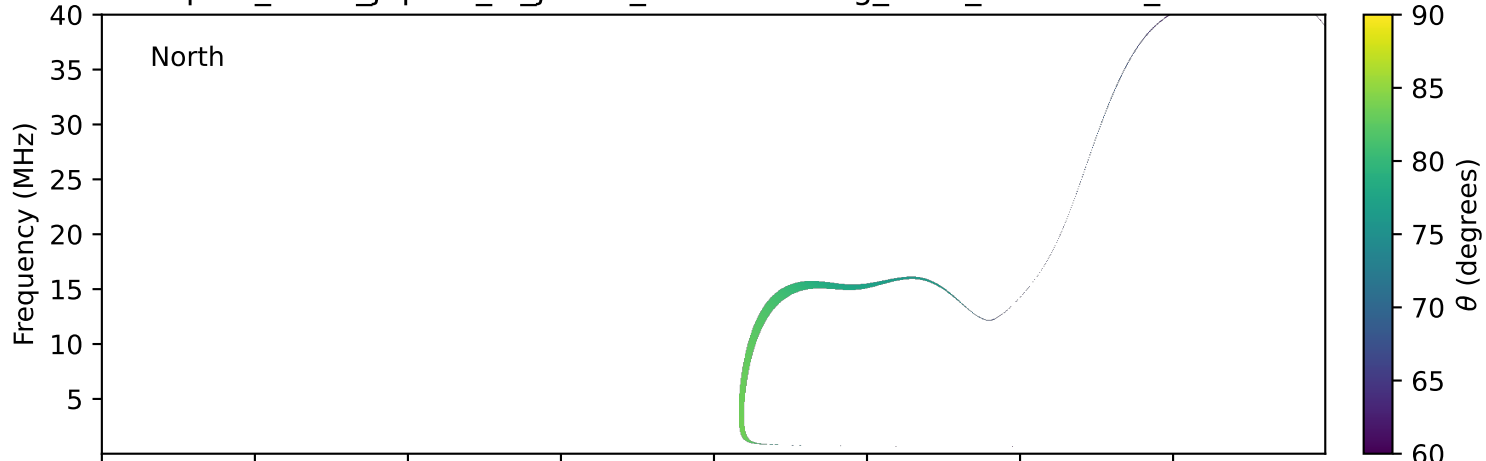
expres_earth_jupiter_io_jrm33_lossc-wid1deg_3kev_20280904_v11.cdf
