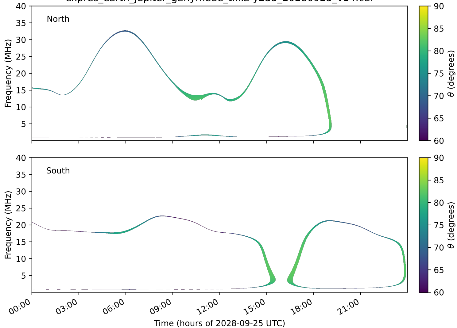
expres_earth_jupiter_ganymede_txka-y235_20280925_v14.cdf
