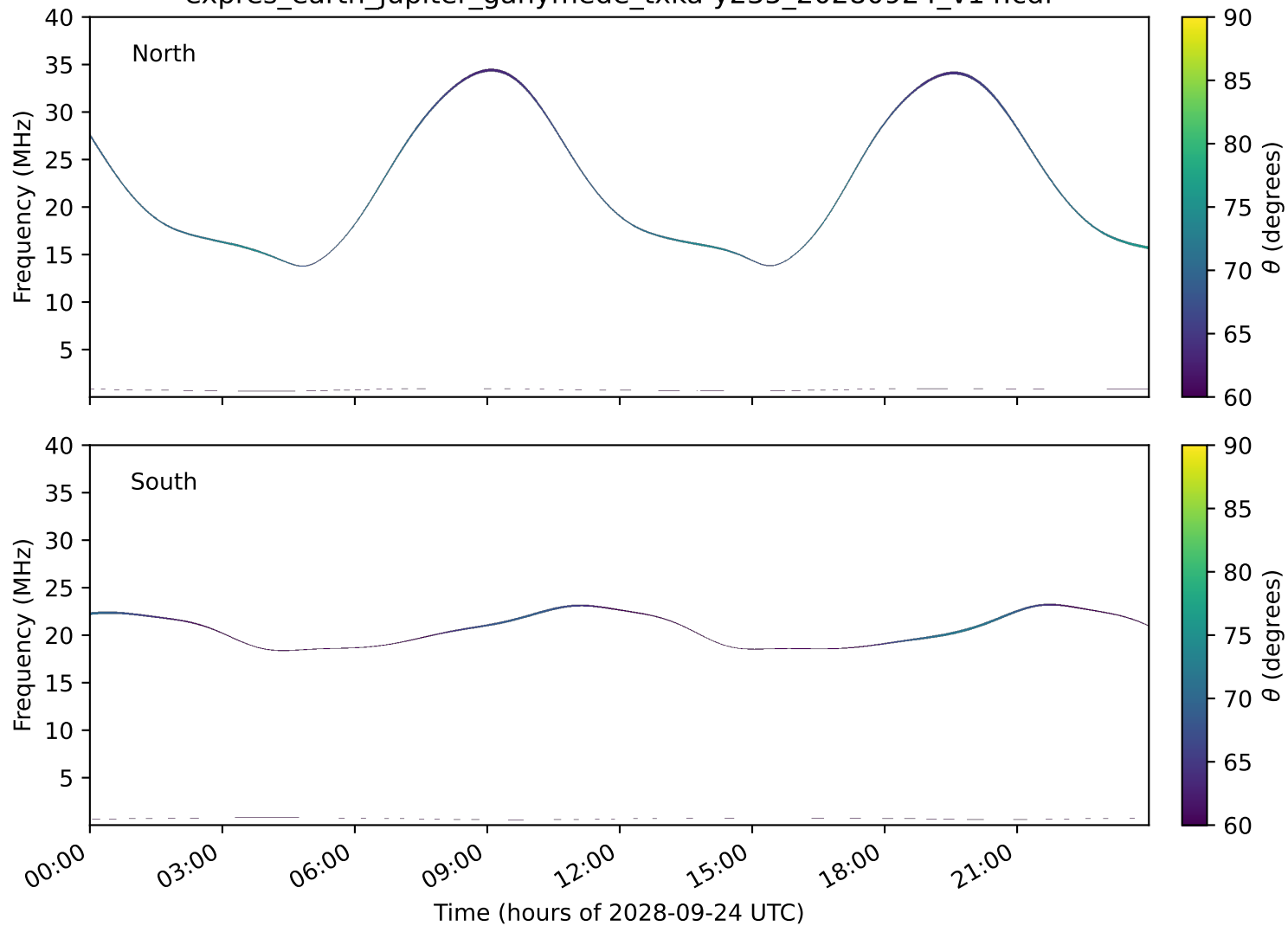
expres_earth_jupiter_ganymede_txka-y235_20280924_v14.cdf
