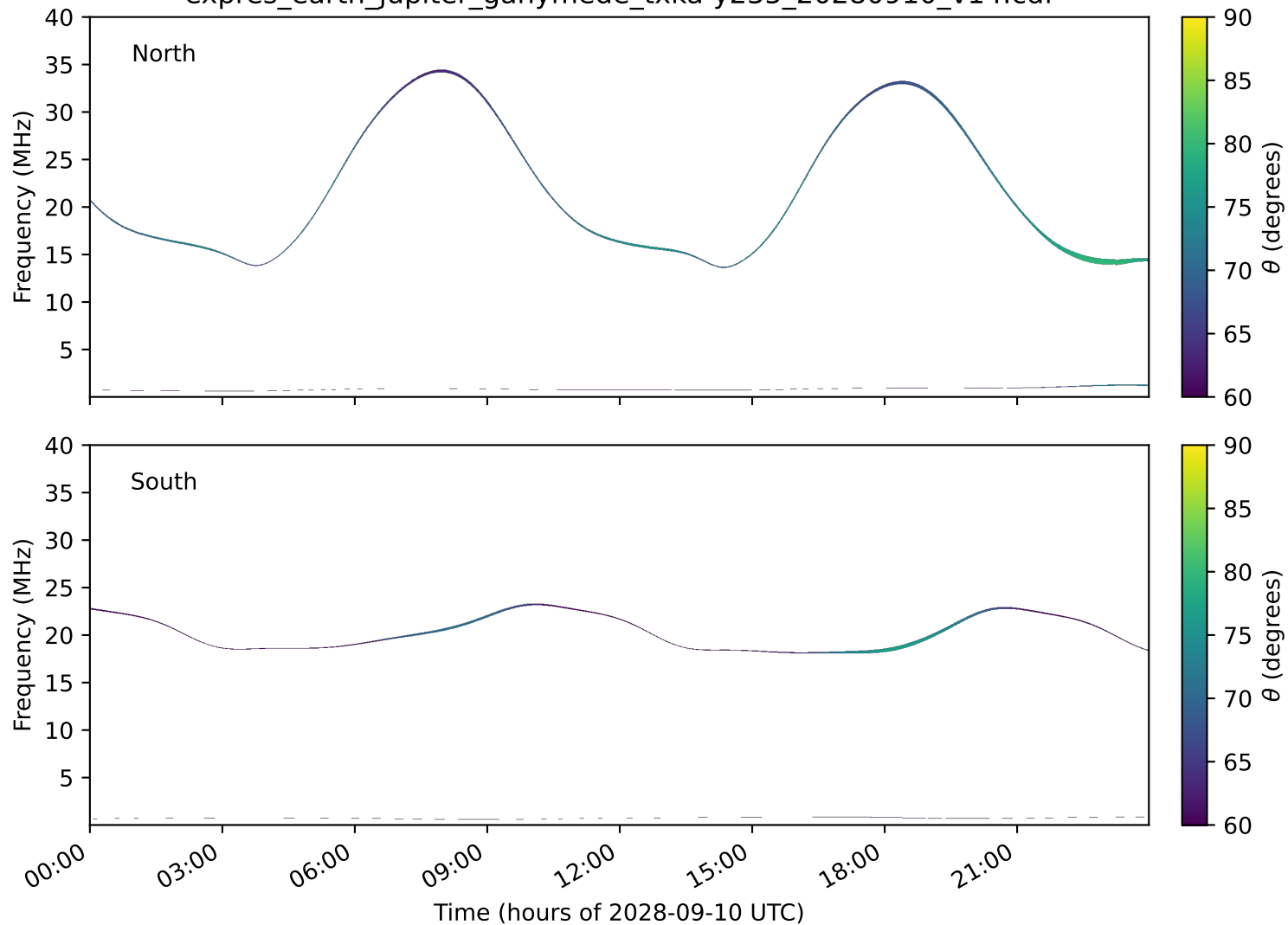
expres_earth_jupiter_ganymede_txka-y235_20280910_v14.cdf
