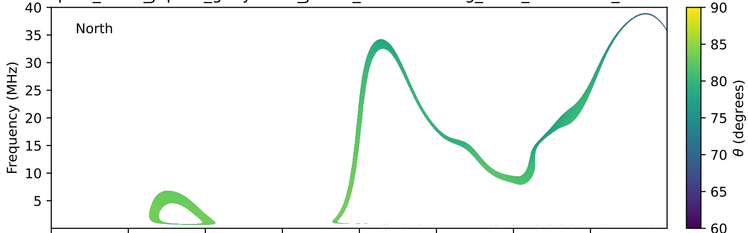
expres_earth_jupiter_ganymede_jrm33_lossc-wid1deg_3kev_20280930_v11.cdf
