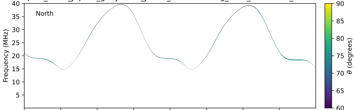
expres_earth_jupiter_ganymede_jrm33_lossc-wid1deg_3kev_20280910_v11.cdf
