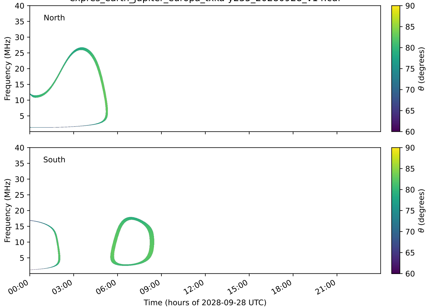
expres_earth_jupiter_europa_txka-y235_20280928_v14.cdf
