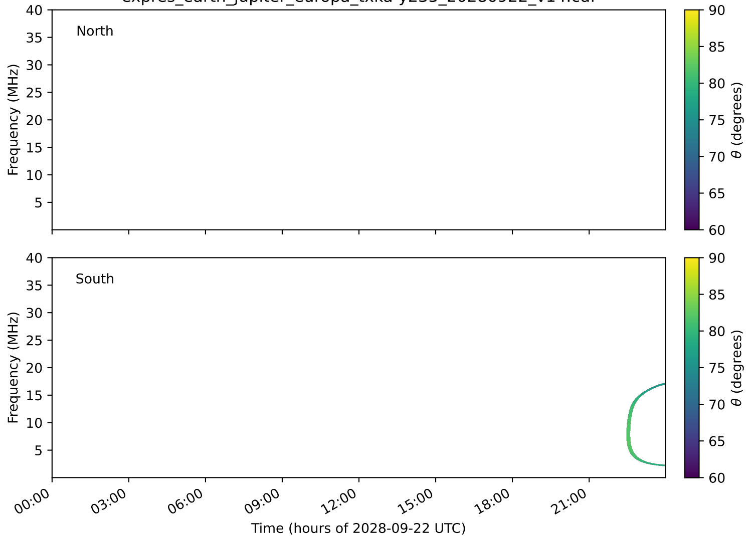
expres_earth_jupiter_europa_txka-y235_20280922_v14.cdf
