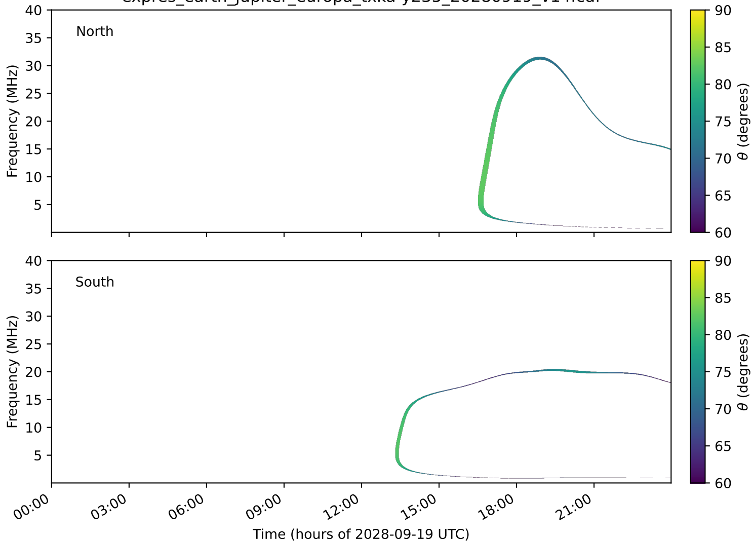
expres_earth_jupiter_europa_txka-y235_20280919_v14.cdf
