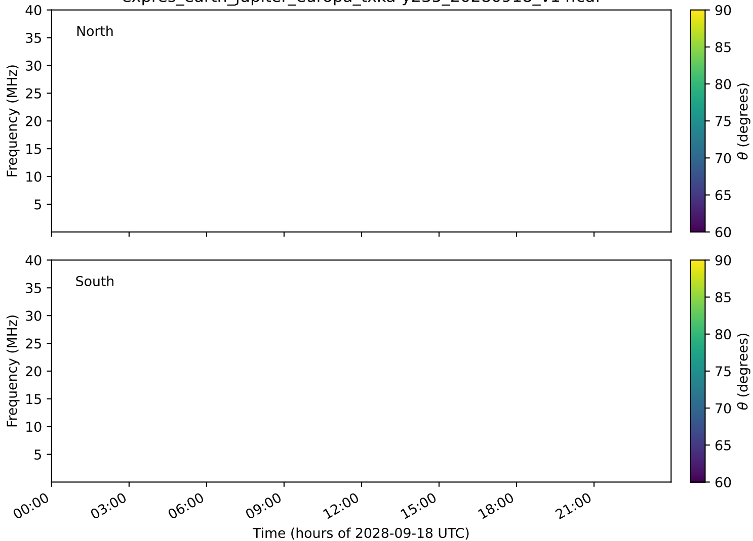
expres_earth_jupiter_europa_txka-y235_20280918_v14.cdf
