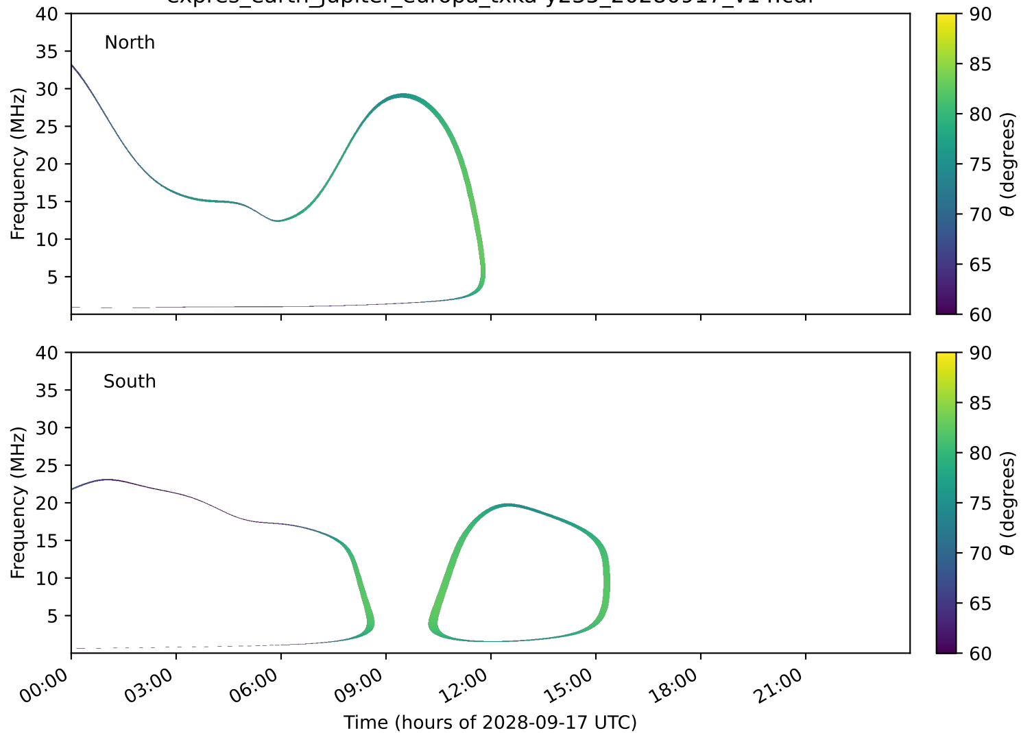
expres_earth_jupiter_europa_txka-y235_20280917_v14.cdf
