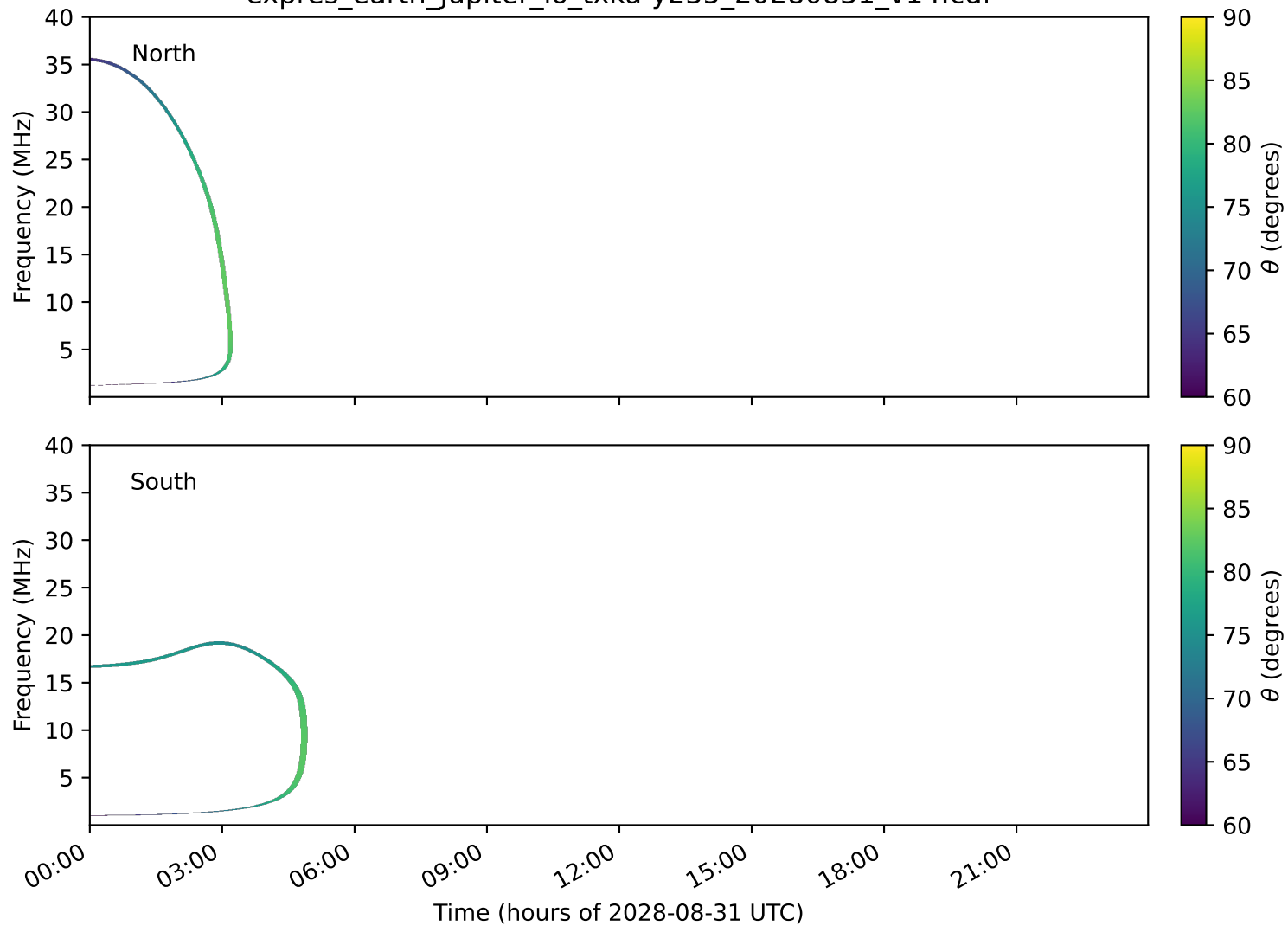
expres_earth_jupiter_io_txka-y235_20280831_v14.cdf
