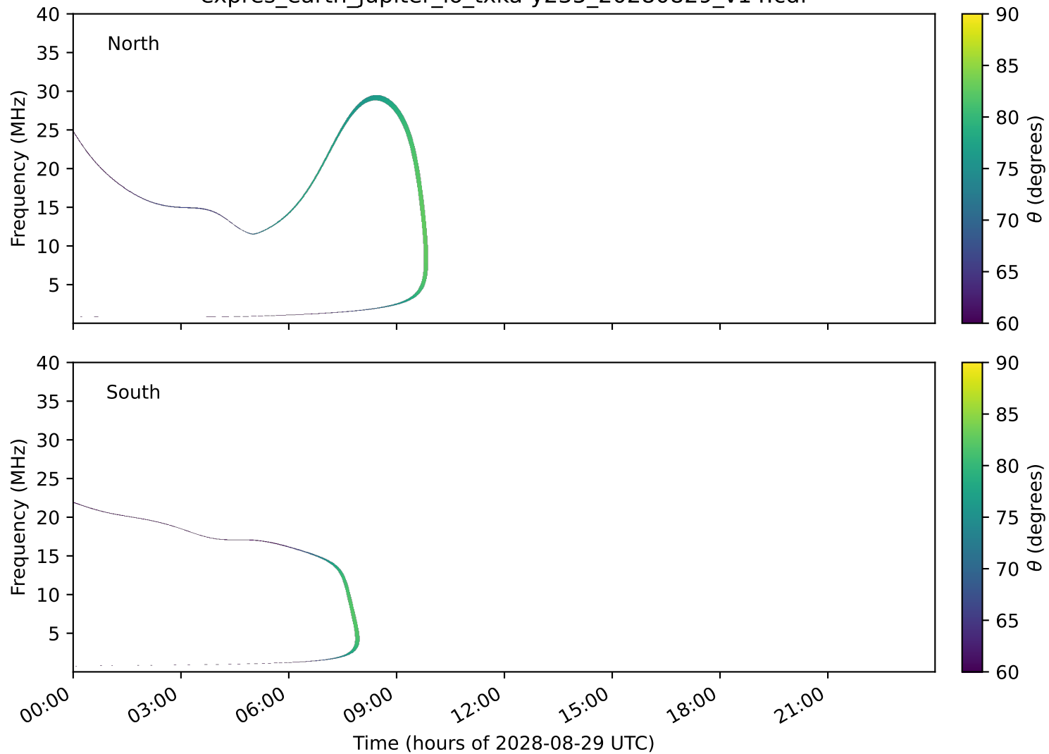
expres_earth_jupiter_io_txka-y235_20280829_v14.cdf
