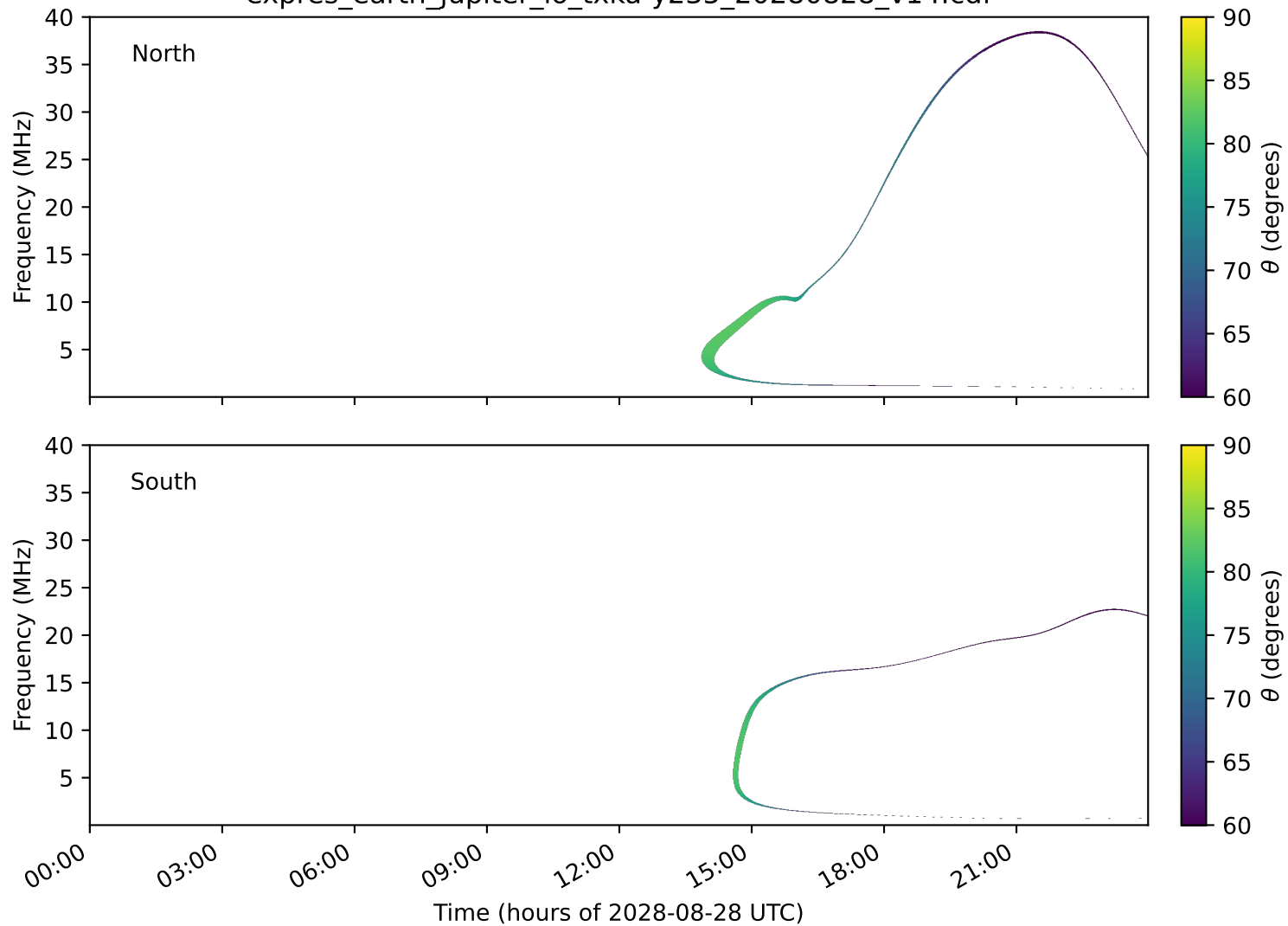
expres_earth_jupiter_io_txka-y235_20280828_v14.cdf
