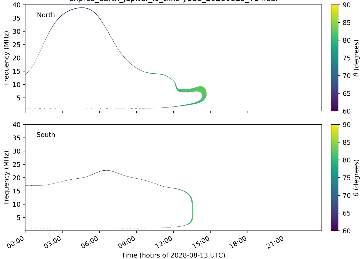
expres_earth_jupiter_io_txka-y235_20280813_v14.cdf
