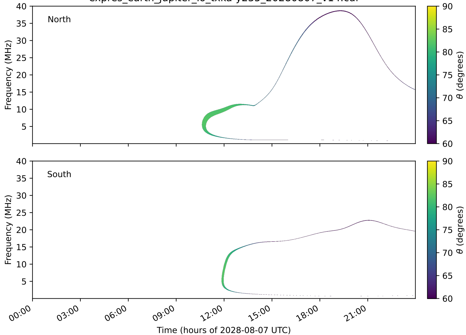
expres_earth_jupiter_io_txka-y235_20280807_v14.cdf
