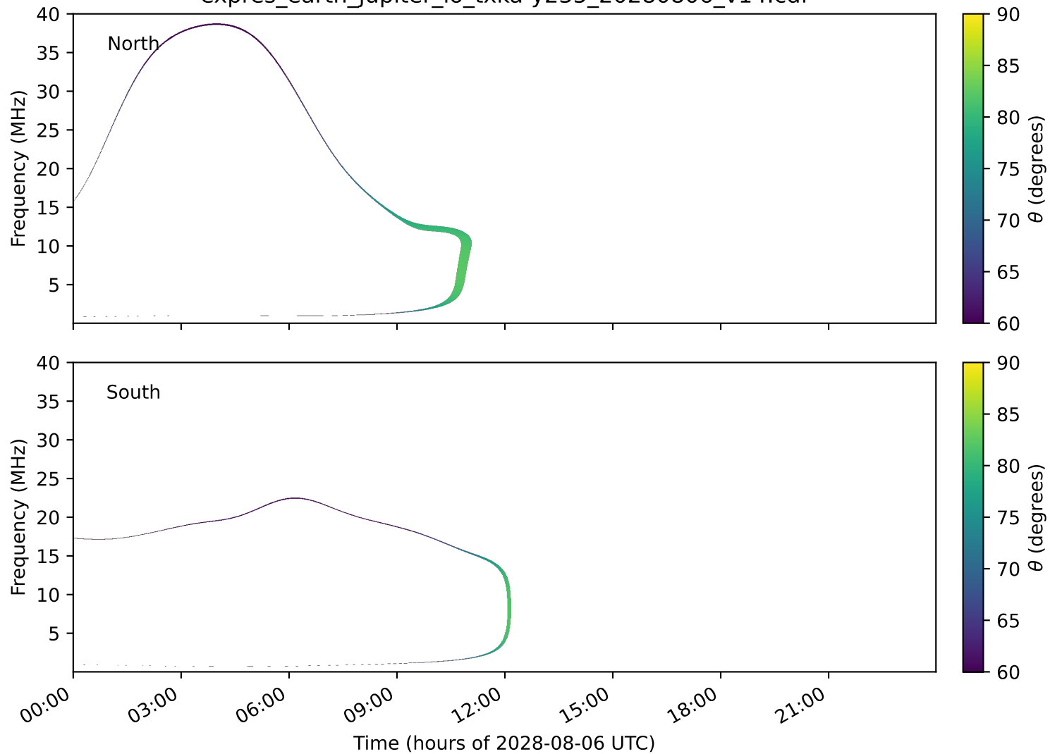
expres_earth_jupiter_io_txka-y235_20280806_v14.cdf
