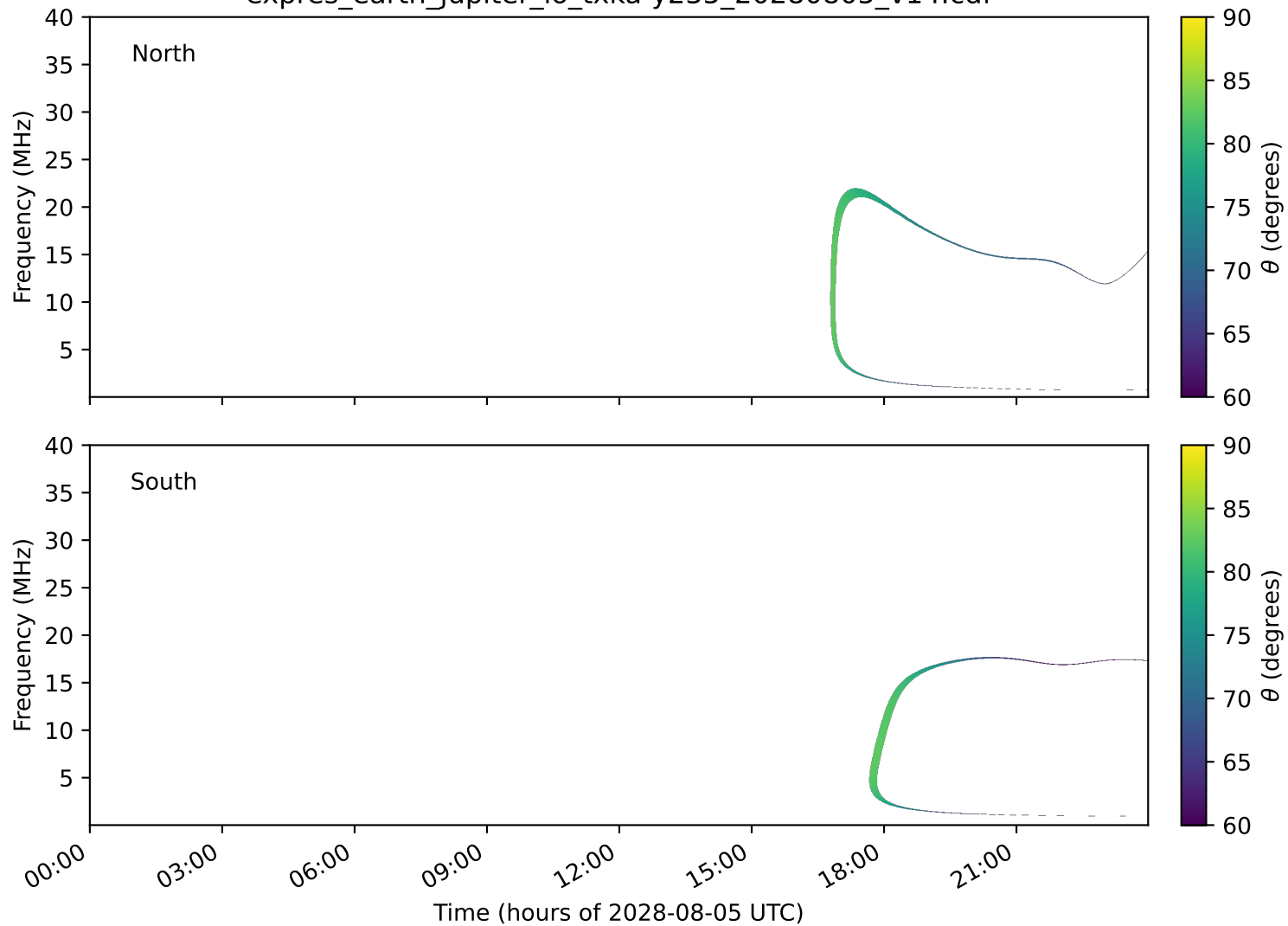
expres_earth_jupiter_io_txka-y235_20280805_v14.cdf
