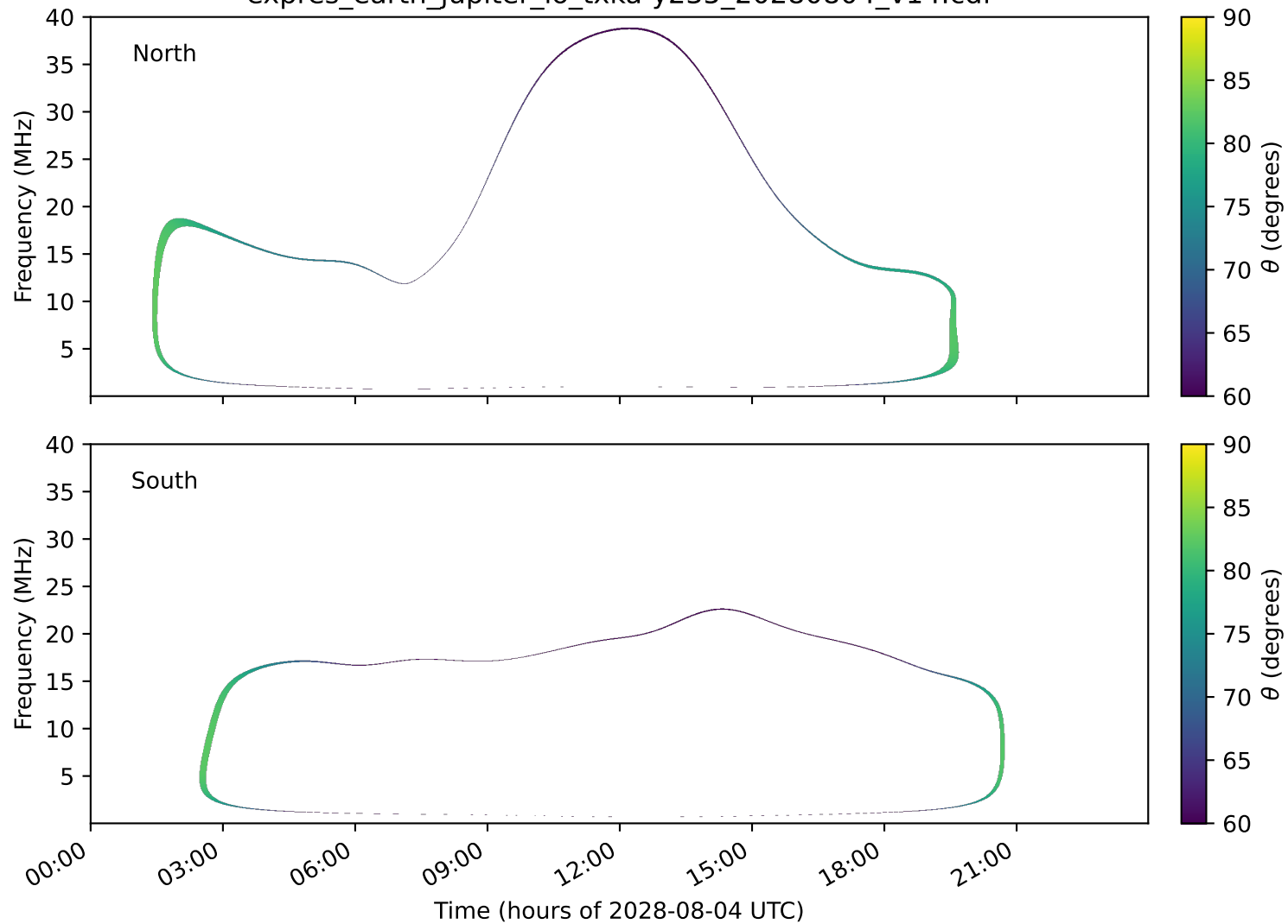
expres_earth_jupiter_io_txka-y235_20280804_v14.cdf
