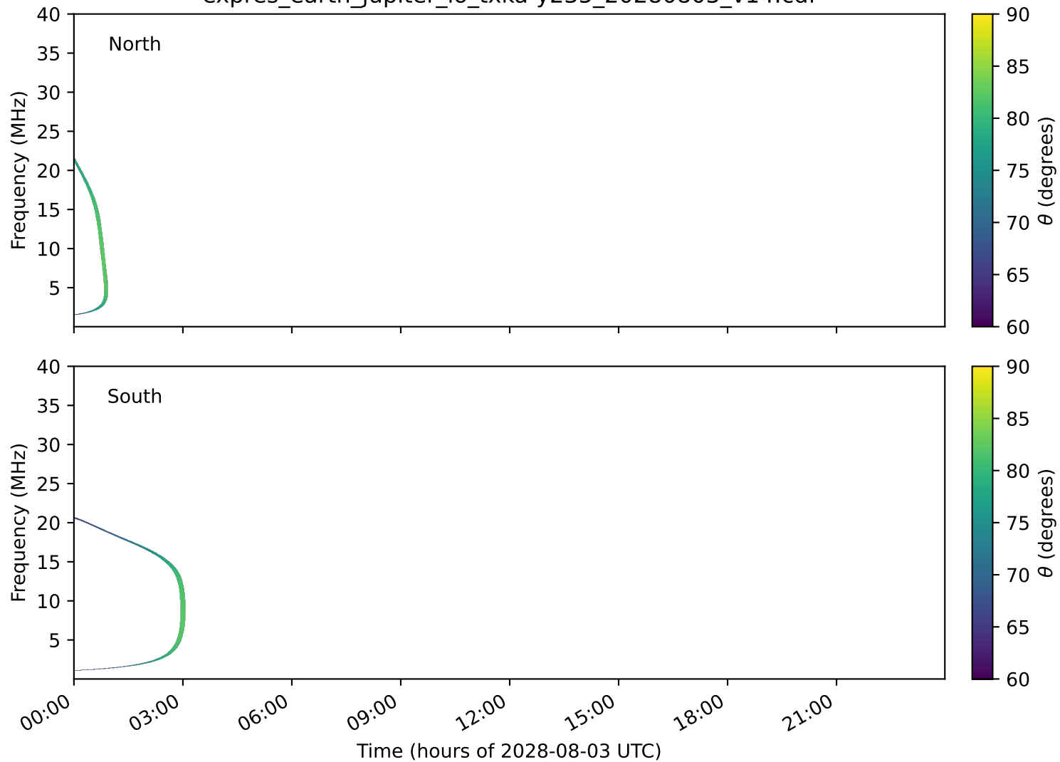
expres_earth_jupiter_io_txka-y235_20280803_v14.cdf
