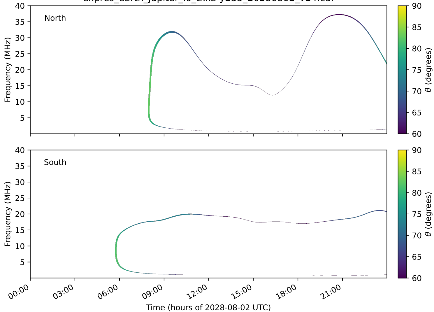
expres_earth_jupiter_io_txka-y235_20280802_v14.cdf
