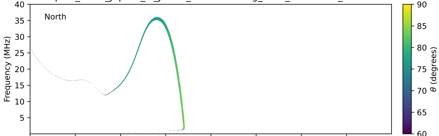
expres_earth_jupiter_io_jrm33_lossc-wid1deg_3kev_20280829_v11.cdf
