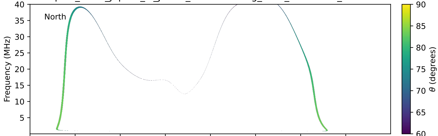
expres_earth_jupiter_io_jrm33_lossc-wid1deg_3kev_20280825_v11.cdf
